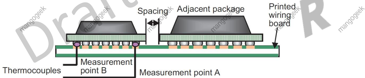
Figure 9-2 Measuring the Reflow Soldering Process
