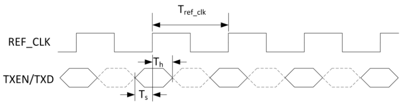
Figure 5-12 RMII Interface Transmit Timing
