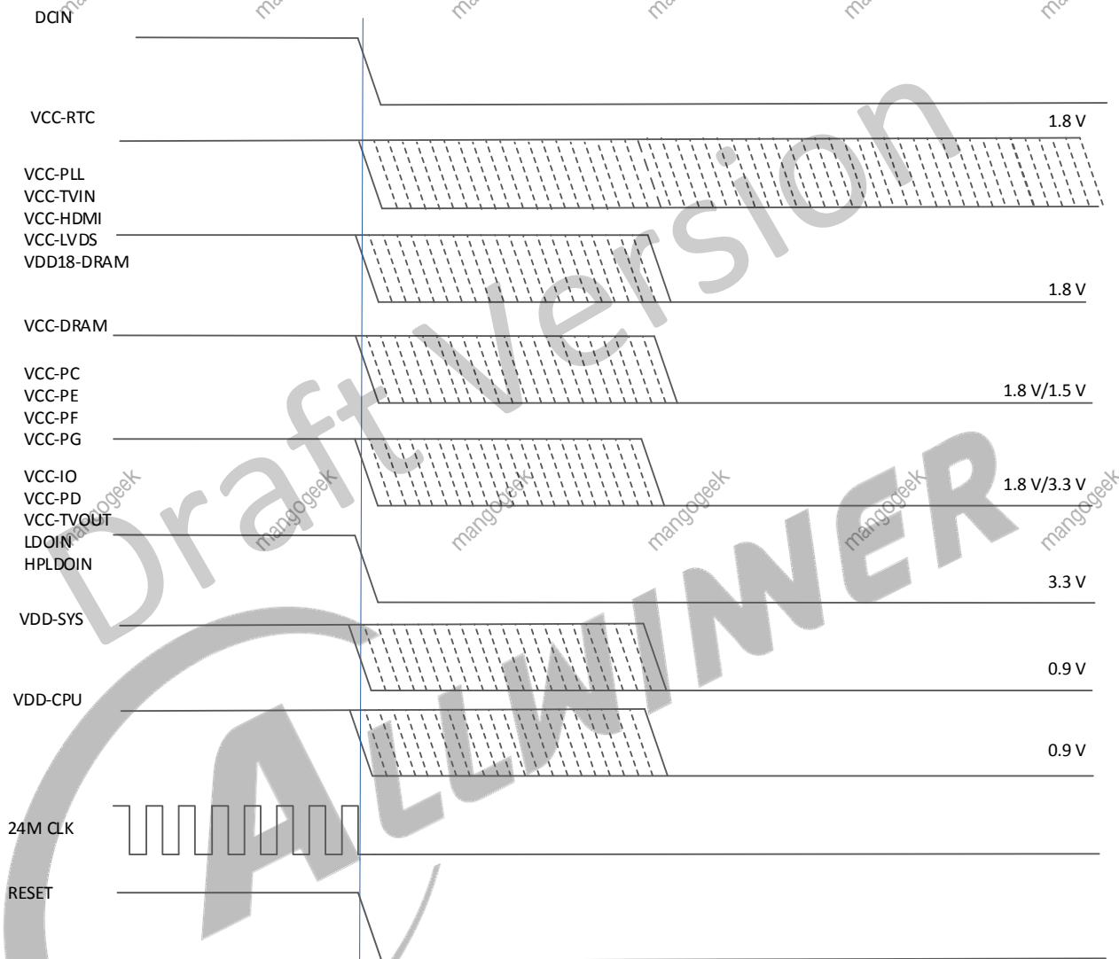
Figure 5-26 Power-Off Timing
